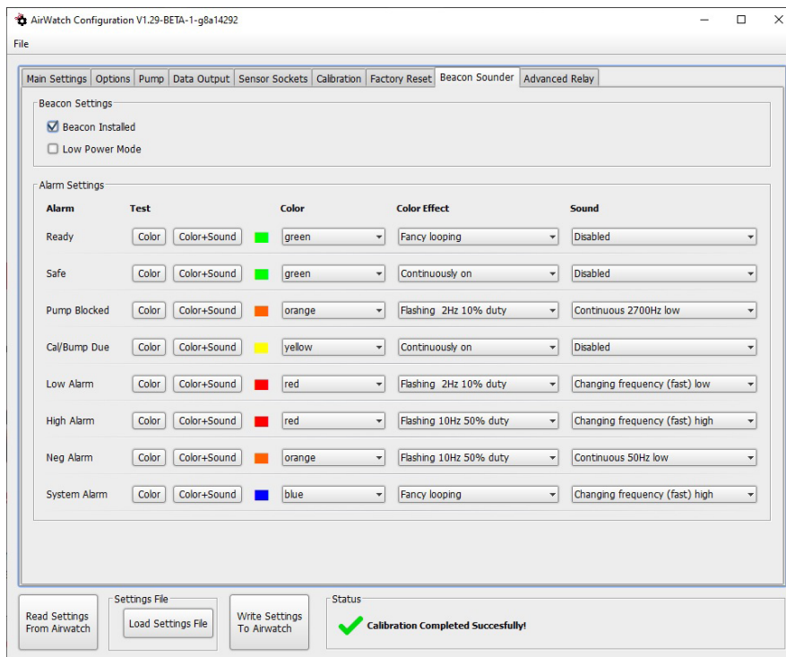
Configurator Beacon Sounder
