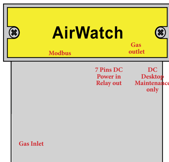
Bottom of AirWatch with Gas inlet, Modbus, 7Pins DC Power in Relay out, Gas outlet & DC Desktop (Maintenance only)
