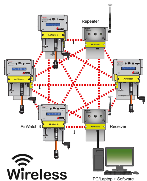
Wireless AirWatch mesh network with one receiver, one repeater and four AirWatches.
