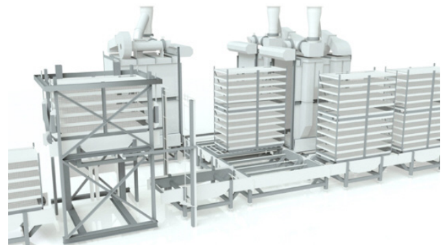
Figure 1: Multistage CO 2 stunning system for poultry
