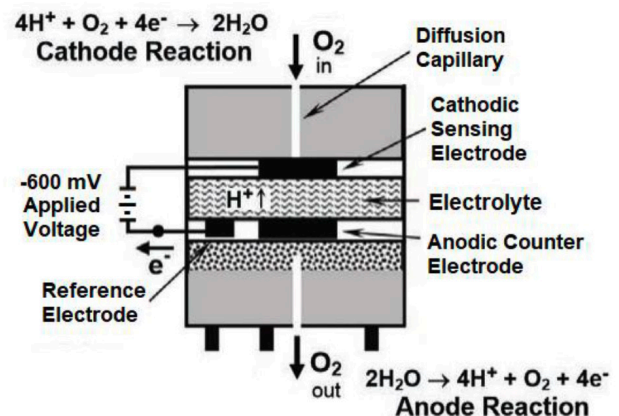
Catalytic Lead-Free Oxygen Sensor
